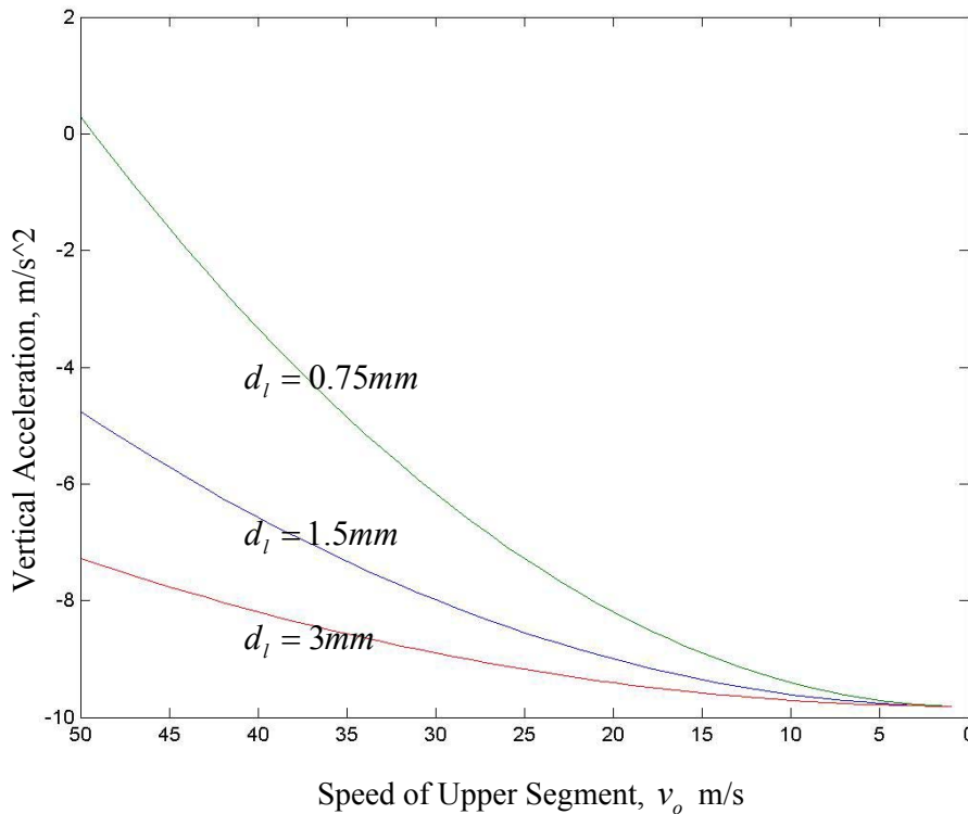
Figure 7. The vertical acceleration of the loop front as the cast unfolds from high speed to low speed. Results are shown for an example floating line for three different line diameters. These results can also be used to predict the effect of line density as explained below.
