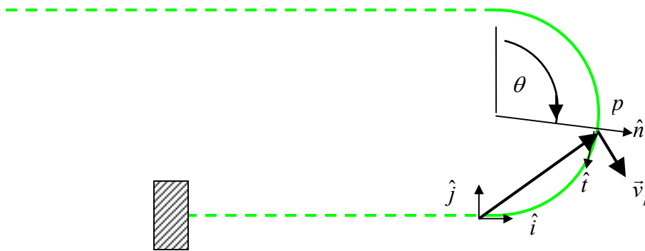
Figure 5. The velocity at point p is resolved into components along the local tangential and normal (\hat{t}, \hat{n}) .
